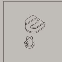
Spansteun set "in de dag" Scala 50 (50 mm) & Retro (50 mm) 2080 2030 aluminium
